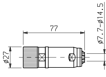
PLUG 220065R1610/1611
